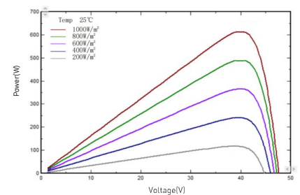
I-V/P-V Curve at Different Irradiation (630W)
